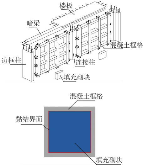
图 1 密肋复合墙体结构体系构造示意 Fig.1 Multi-ribbed wall structure
